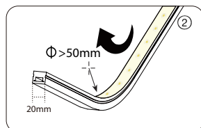
2. Correct bending way
